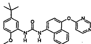
1-(5-tert-Butyl-2-methoxy-phenyl)-3-[4-(pyrimidin-4-yloxy)-naphthalen-1-yl]-urea;
